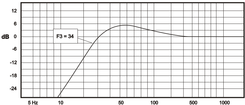
QC12S4 AMPLITUDE RESPONSE (DB/HZ)
